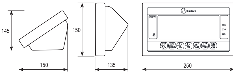
Dimensions (mm)
